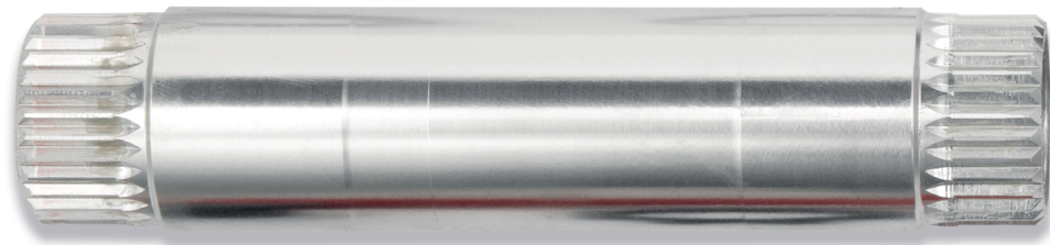
Axle 133.5mm (68/73) HC108-07 148.5mm (83) HC108-08 165.5mm (100) HC108-09 185.5mm (120) HC108-10
